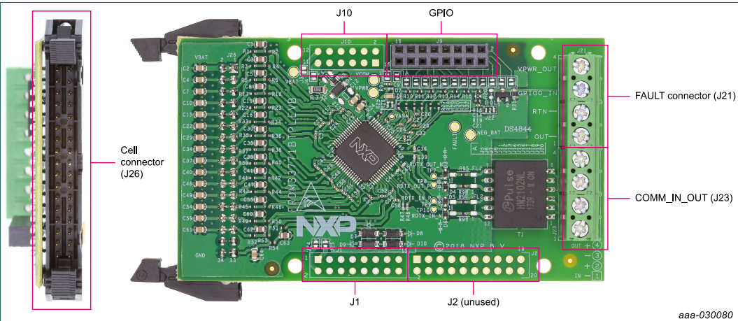
Figure 5. Connectors
