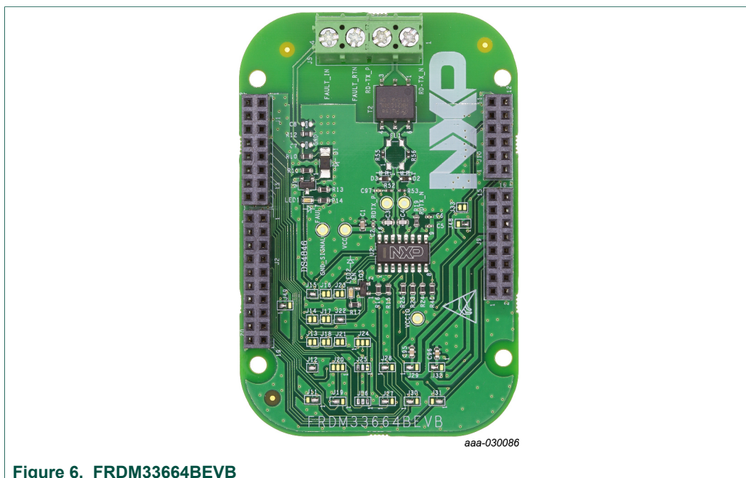
Figure 6. FRDM33664BEVB
