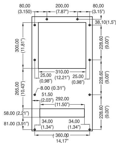
Drilling Template
