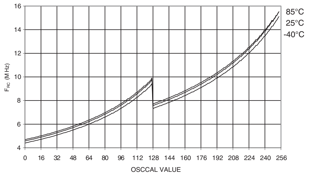
Figure 27-57. Calibrated 8 MHz RC Oscillator Frequency vs. OSCCAL Value
