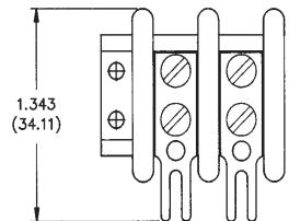
"3/4W" Terminals
