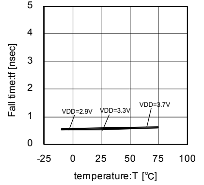
Fig.36 54MHz Fall-time temperature characteristics
