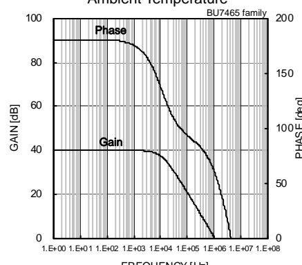
Fig.92 Gain – Frequency
