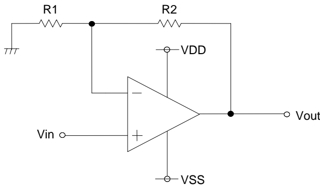
Fig.192 Non-inverting amplifier
