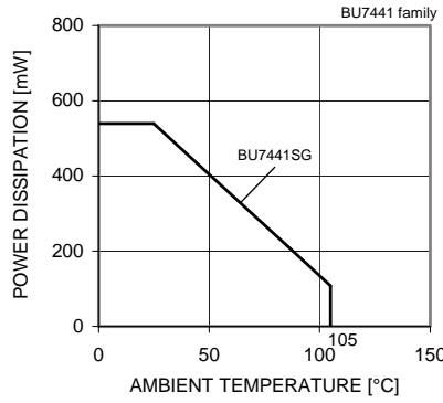
Fig.94 Derating curve
