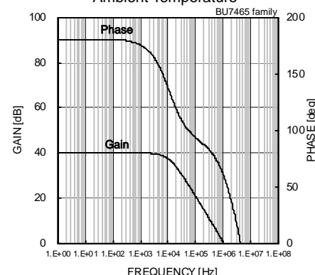
Fig.92 Gain – Frequency
