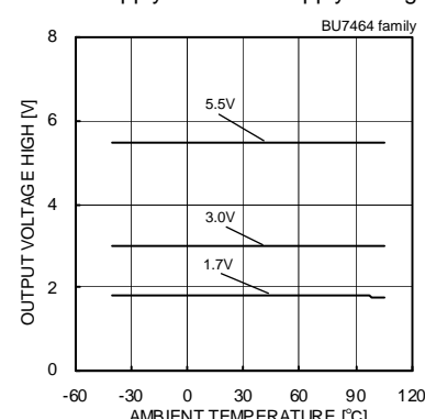
Fig.52 Output Voltage High - Ambient Temperature ( R_L=10[k\Omega] )
