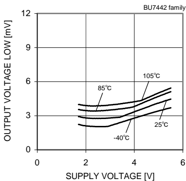
Fig.122 Output Voltage Low – Supply Voltage ( R_L=10[k\Omega] )
