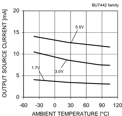
Fig.125 Output Source Current – Ambient Temperature ( V_{OUT}=V_{DD}-0.4[V] )
