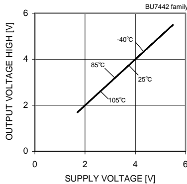
Fig.120 Output Voltage High – Supply Voltage ( R_L=10[k\Omega] )
