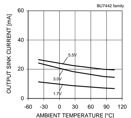
Fig.127 Output Sink Current – Ambient Temperature ( V_{OUT}=V_{SS}+0.4[V] )
