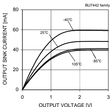
Fig.126 Output Sink Current – Output Voltage ( V_{DD}=3[V] )
