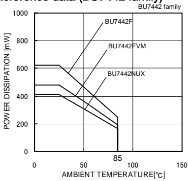
Fig.116 Derating curve
