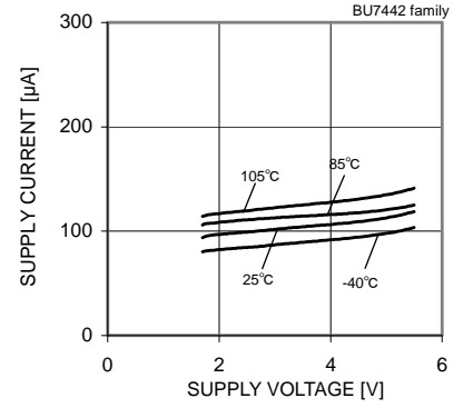
Fig.118 Supply Current – Supply Voltage
