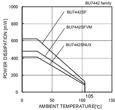
Fig.117 Derating curve
