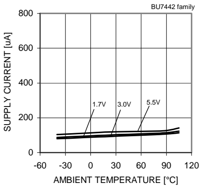
Fig.119 Supply Current – Ambient Temperature
