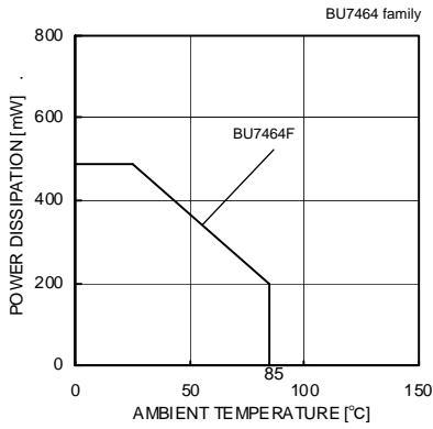
Fig.47 Derating curve
