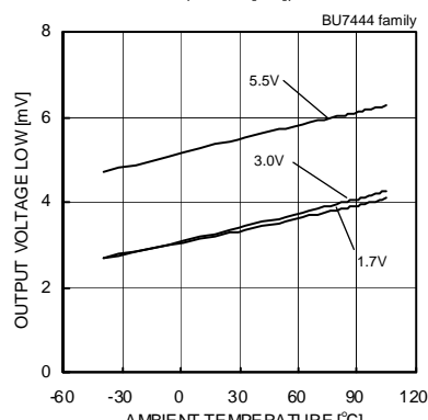
Fig.146 Output Voltage Low - Ambient Temperature (RL=10[kΩ])
