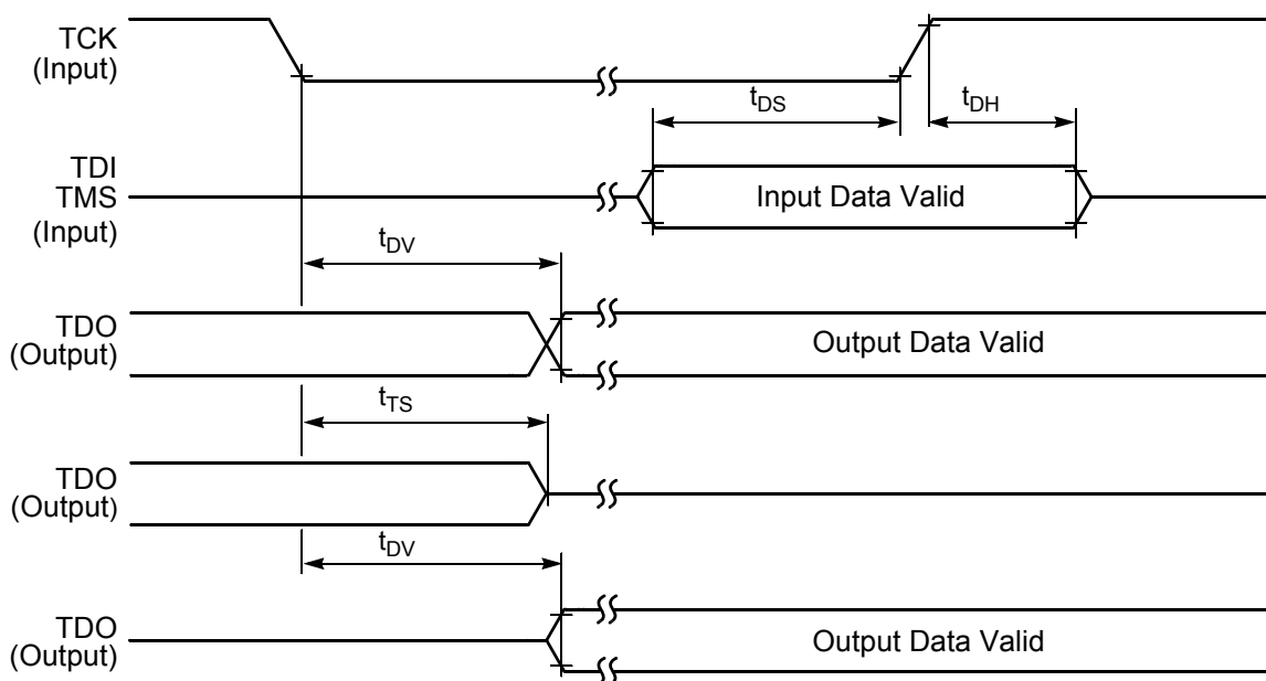
Figure 3-31 Test Access Port Timing Diagram
