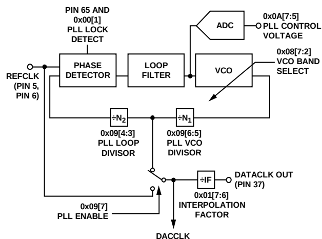
Figure 72. Clock Multiplier Circuit
