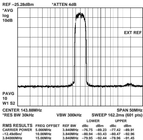
Figure 32. AD9779A W-CDMA Signal, 4x Interpolation, f_{DATA} = 122.88 MSPS, f_{DAC}/4 Modulation
