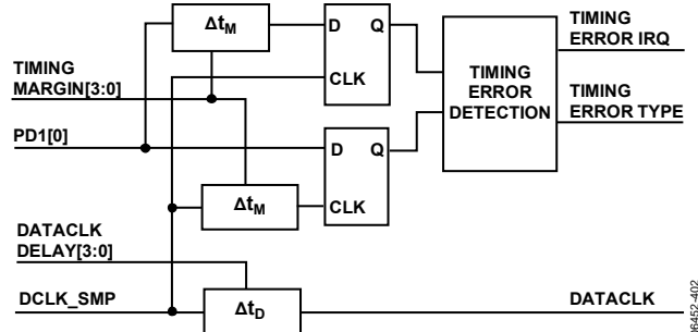
Figure 86. Timing Error Detection and Optimization Circuitry
