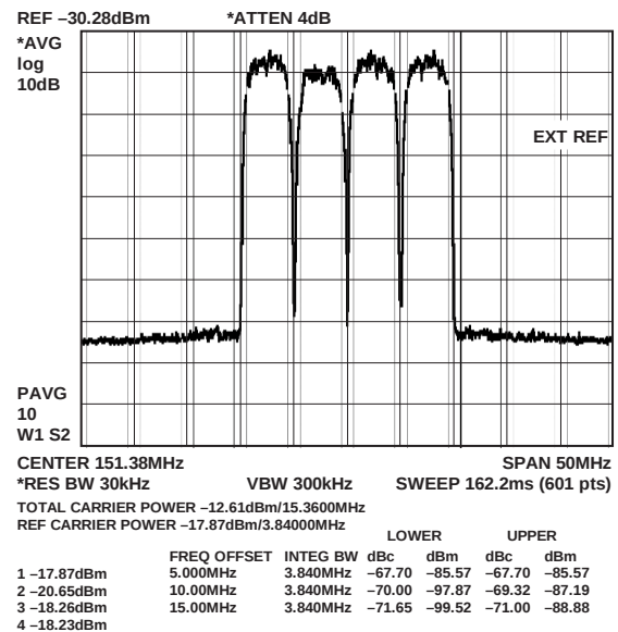
Figure 35. AD9779A Multicarrier W-CDMA Signal, 4\times Interpolation, f_{DAC} = 122.88 MSPS, f_{DAC}/4 Modulation
