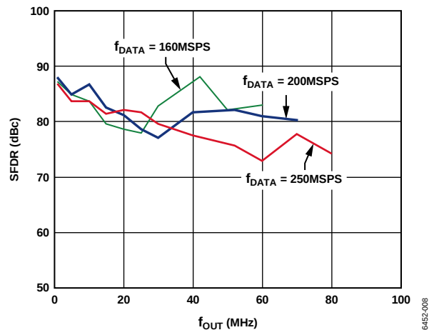
Figure 9. AD9779A In-Band SFDR vs. f_{OUT} , 2 \times Interpolation
