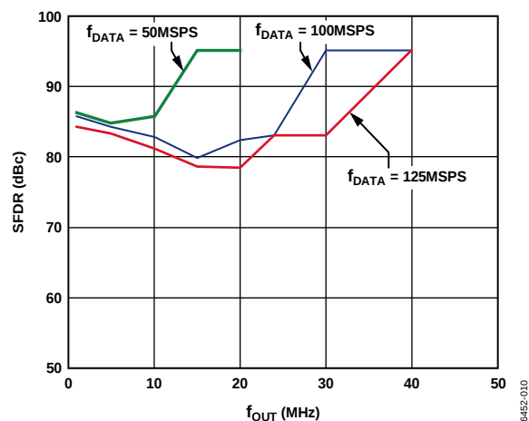
Figure 11. AD9779A In-Band SFDR vs. f_{OUT} , 8 \times Interpolation
