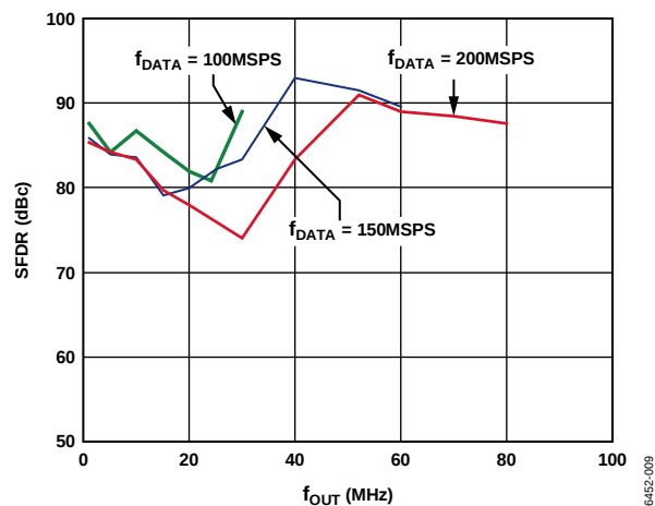
Figure 10. AD9779A In-Band SFDR vs. f_{OUT} , 4 \times Interpolation
