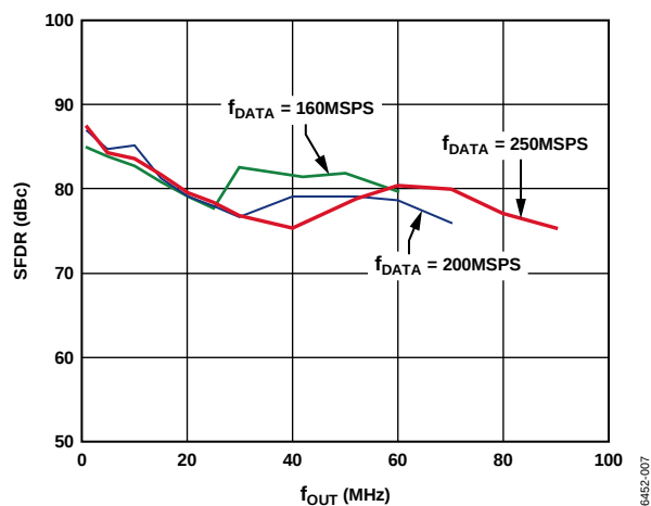
Figure 8. AD9779A In-Band SFDR vs. f_{OUT} , 1 \times Interpolation
