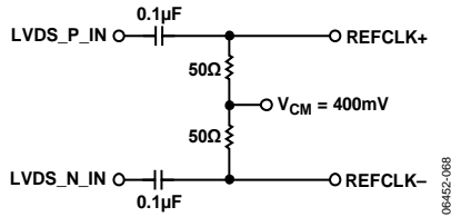
Figure 73. LVDS REFCLK Drive Circuit
