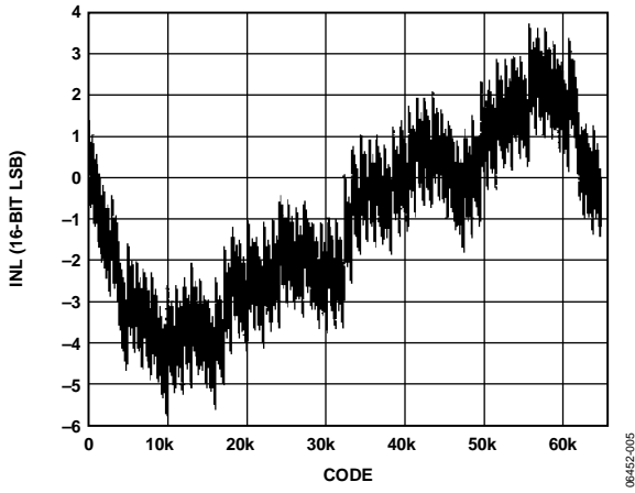
Figure 6. AD9779A Typical INL
