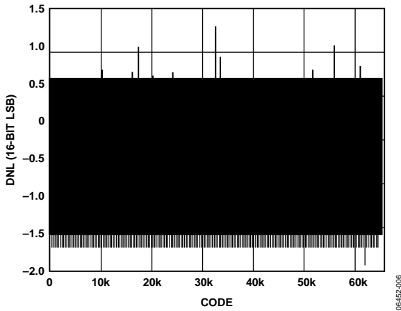
Figure 7. AD9779A Typical DNL
