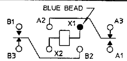
TERMINAL VIEW
