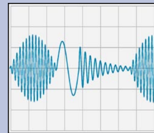
Waveform sequencing
