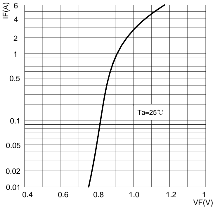
FIG3: Forward Voltage
