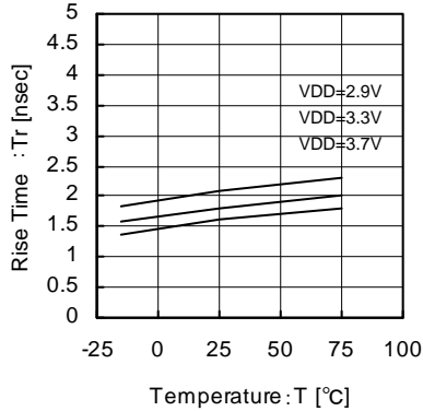
Fig.28 33.8688MHz Temperature - rise-time
