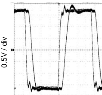
Fig.25 Buffer delay(IN→OUT1) VDD=3.3V,CL=50pF
