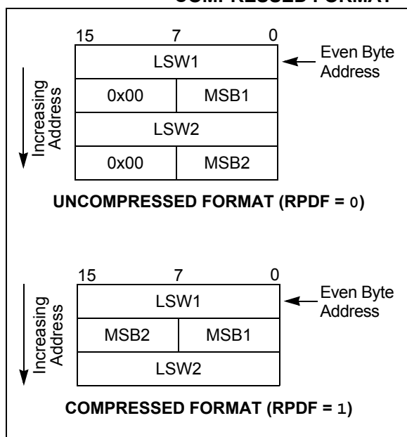
FIGURE 4-14: UNCOMPRESSED/COMPRESSED FORMAT
