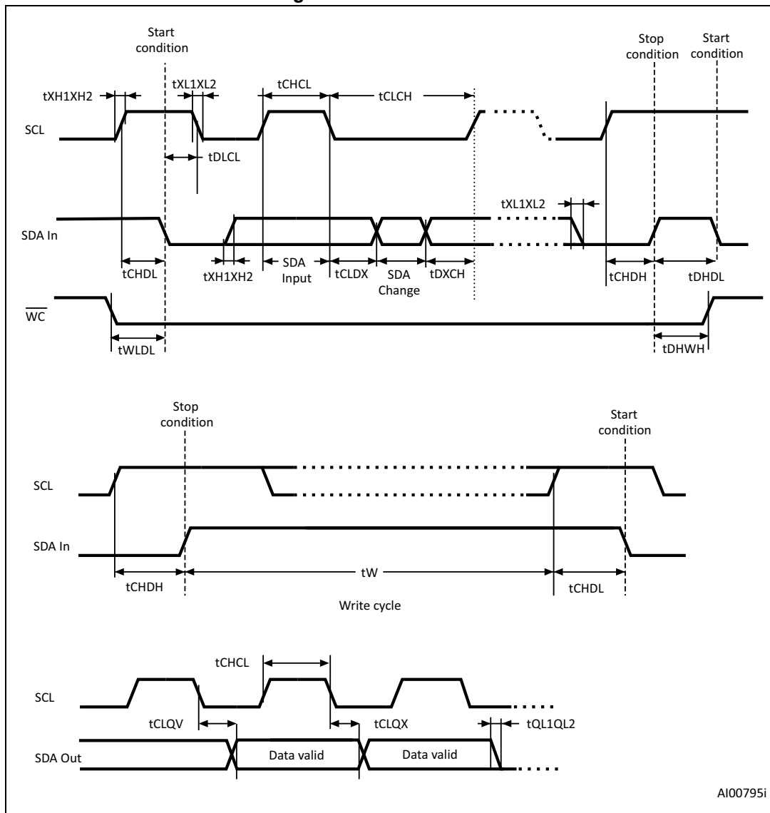
Figure 17. AC waveforms
