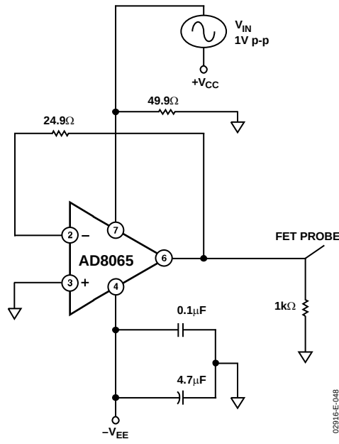
Figure 48. Positive PSRR
