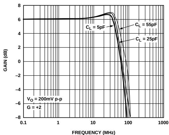
Figure 13. Small Signal Frequency Response for Various C_{LOAD} (See Figure 43)
