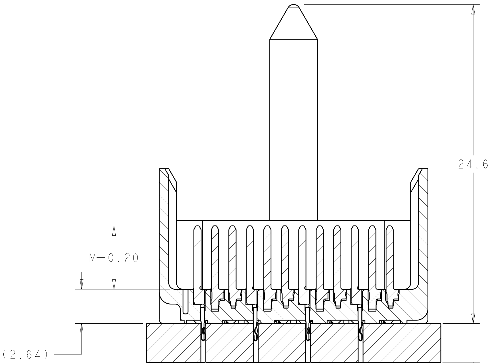
SECTION X-X
