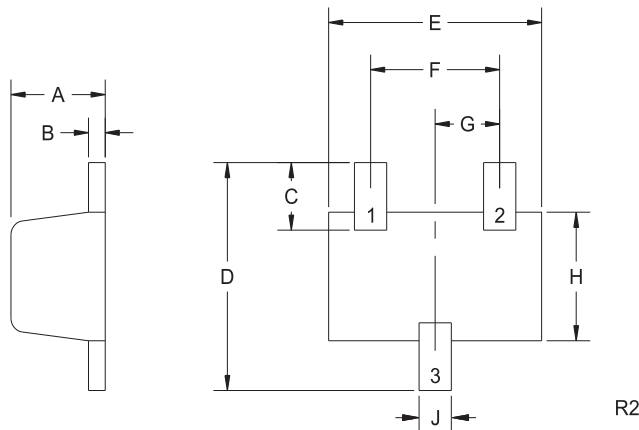
PIN CONFIGURATION (Bottom View)
