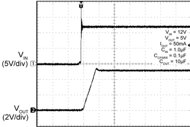
Time (200µs/div)
