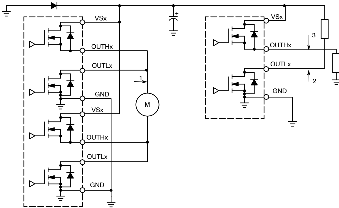
Figure 5. Application Drawing
