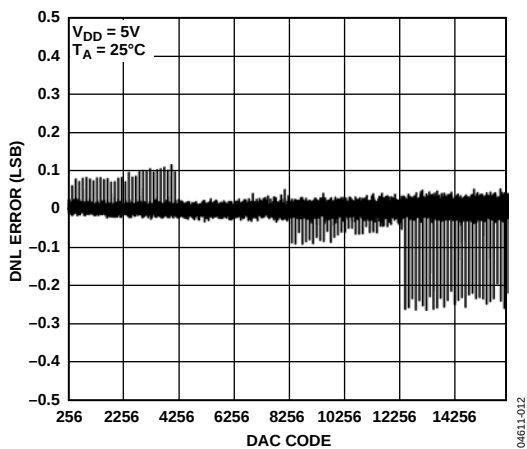
Figure 13. Typical DNL
