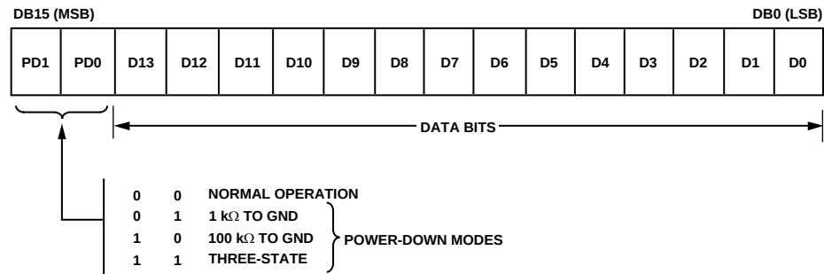
Figure 35. Input Register Contents
