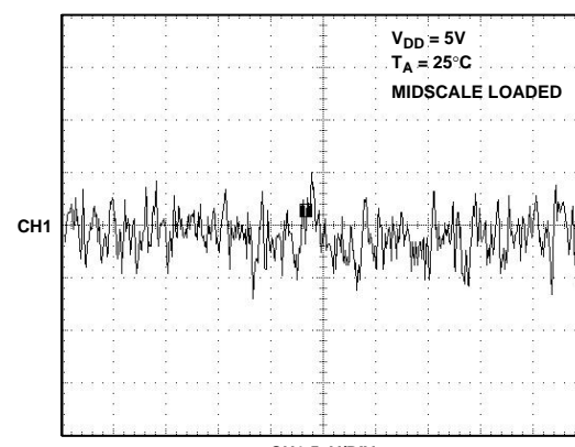
Figure 28. 1/f Noise, 0.1 Hz to 10 Hz Bandwidth
