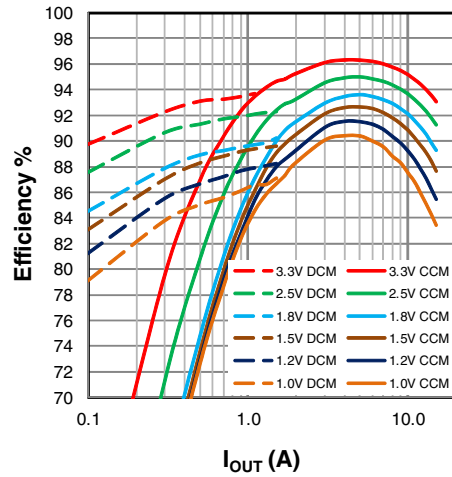
Figure 19: Efficiency, V_{\text{IN}}=5\text{V}
