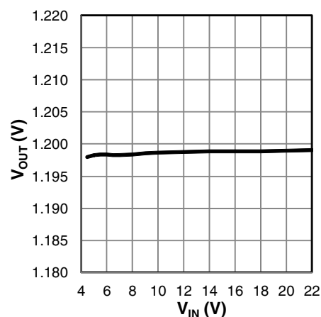
Line Regulation
