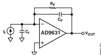
Figure 61. Transimpedance Configuration
