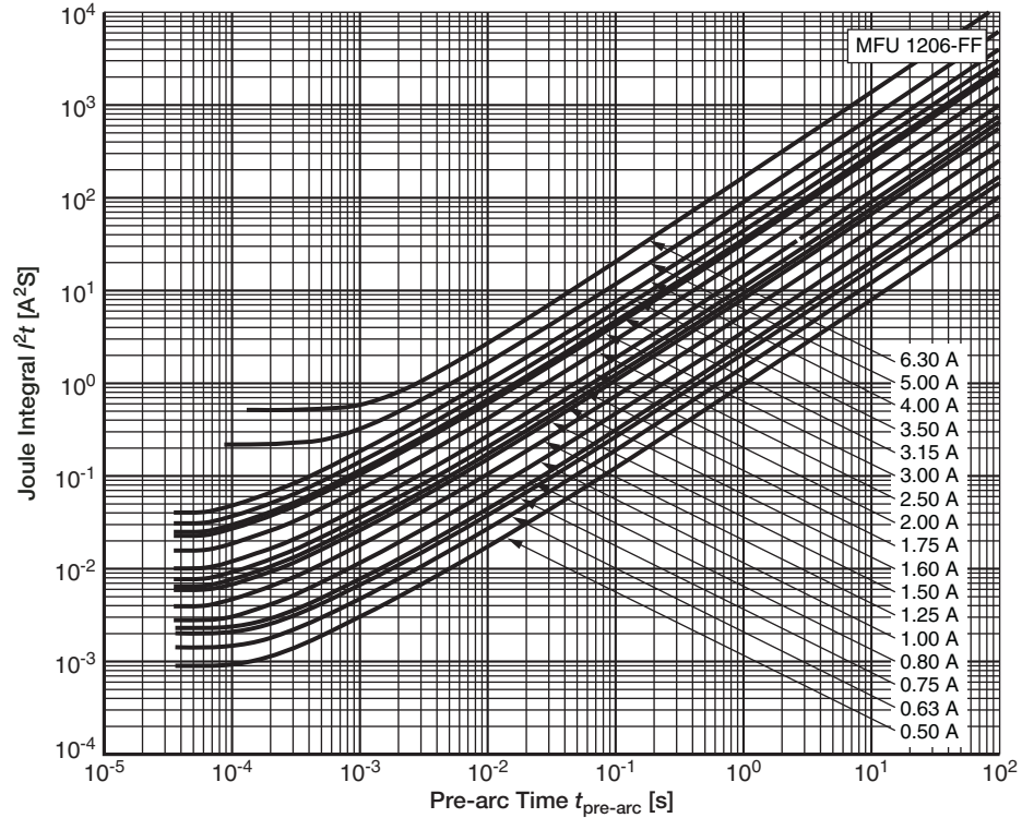
Typical I^2t vs. t_{pre-arc} characteristic of MFU 1206 (1)
