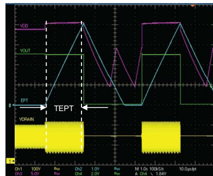
Figure 43. Extra power applied indefinitely
