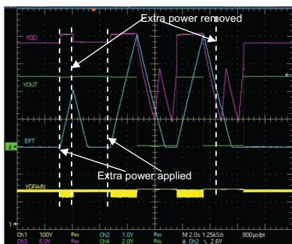
Figure 42. Extra power applied and removed
