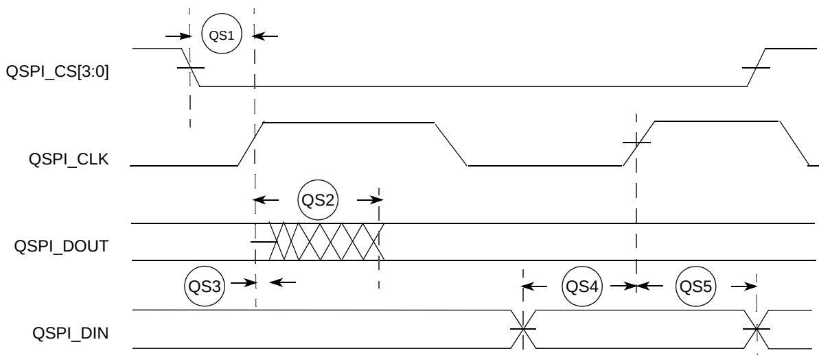
Figure 27. QSPI Timing
