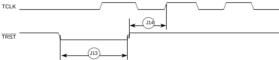
Figure 31. TRST Timing
