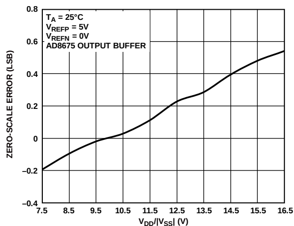
Figure 20. Zero-Scale Error vs. Supply Voltage, 5 V Span
