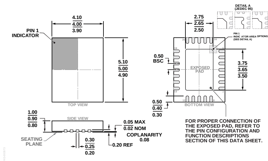
Figure 55. 24-Lead Lead Frame Chip Scale Package [LFCSP] 4 mm x 5 mm Body and 0.90 mm Package Height (CP-24-5) Dimensions shown in millimeters
