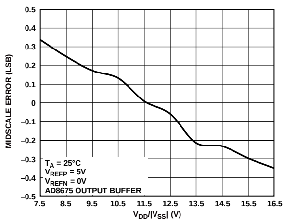
Figure 22. Midscale Error vs. Supply Voltage, 5 V Span
