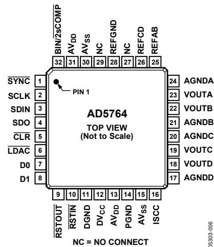
Figure 6. Pin Configuration
