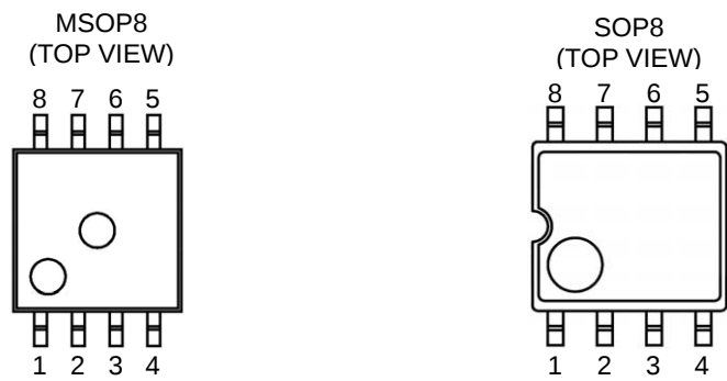
Figure 1. Pin Configurations
