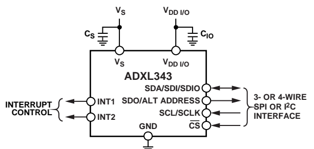
Figure 34. Application Diagram
