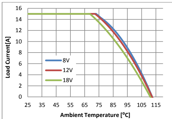
PI3422 - Load Current vs. Ambient Temperature, 0 LFM
