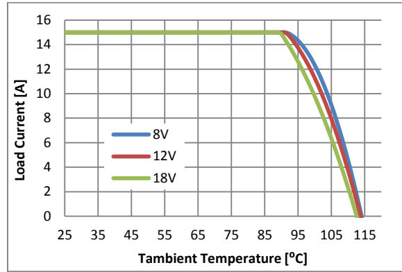
PI3421 - Load Current vs. Ambient Temperature, 0 LFM
