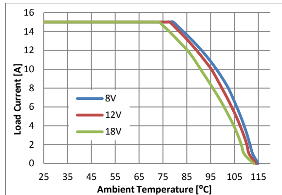
PI3423 - Load Current vs. Ambient Temperature, 0 LFM
