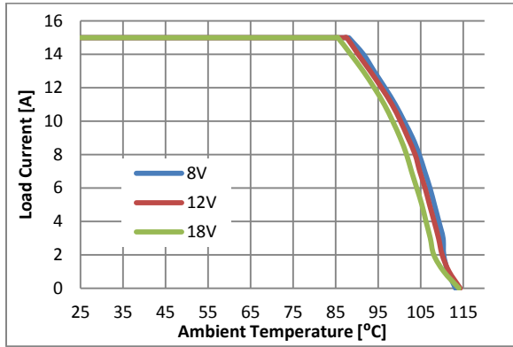
PI3420 - Load Current vs. Ambient Temperature, 0 LFM
