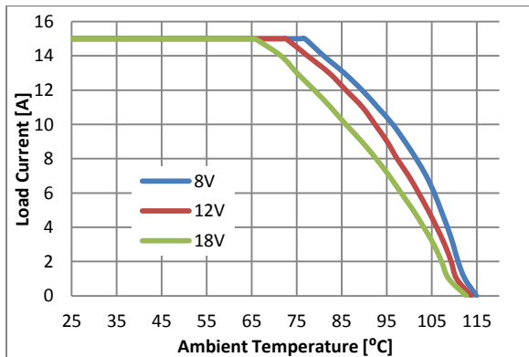
PI3424 - Load Current vs. Ambient Temperature, 0 LFM
