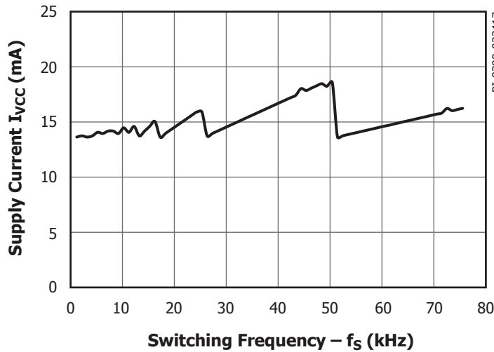
Figure 19. Supply Current Primary-Side I_{VCC} vs. Switching Frequency. Conditions: V_{CC} = 5 V, V_{TOT} = 25 V, T_J = 25 °C, No-Load.
