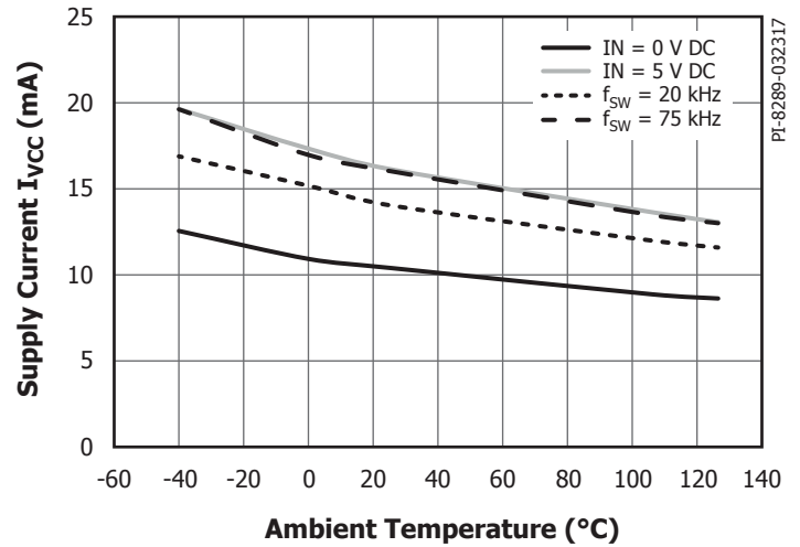
Figure 18. Supply Current Primary-Side I_{VCC} vs. Ambient Temperature. Conditions: V_{CC} = 5 V, V_{TOT} = 25 V, No-Load.
