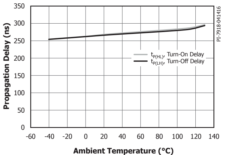
Figure 22. Propagation Delay Time vs. Ambient Temperature. Conditions: V_{CC} = 5 V, V_{TOT} = 25 V, f_S = 20 kHz, C_{LOAD} = 2.2 nF.
