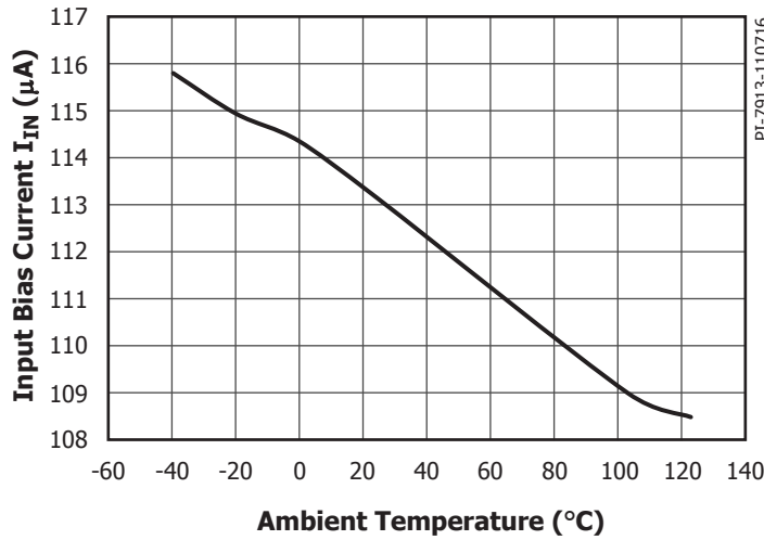
Figure 17. Input Bias Current vs. Ambient Temperature. Conditions: V_{CC} = 5 V, V_{IN} = 5 V, V_{TOT} = 25 V.
