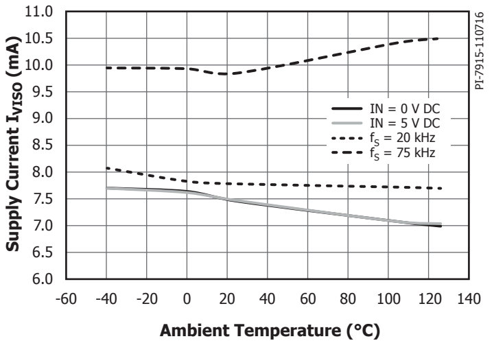
Figure 20. Supply Current Secondary-Side I_{VISO} vs. Ambient Temperature. Conditions: V_{CC} = 5 V, V_{TOT} = 25 V, No-Load.
