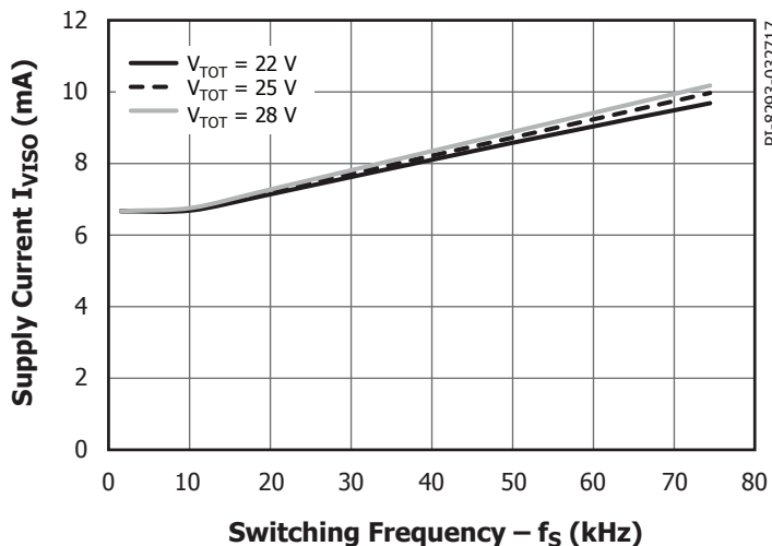
Figure 21. Supply Current Secondary-Side I_{VISO} vs. Switching Frequency. Conditions: V_{CC} = 5 V, No-Load.
