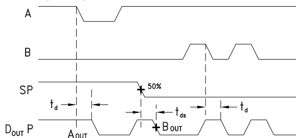
Timing Diagram
