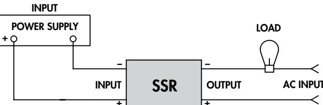
WIRING DIAGRAM
