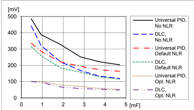
Load transient peak voltage deviation vs. external capacitance. Step (12.5-37.5-12.5 A), Parallel coupling of capacitors with 470 \mu F/10 m \Omega , T_{P1} = +25 °C. V_I = 12 V, V_O = 3.3 V, f_{sw} = 320 kHz, di/dt = 2 A/ \mu s
