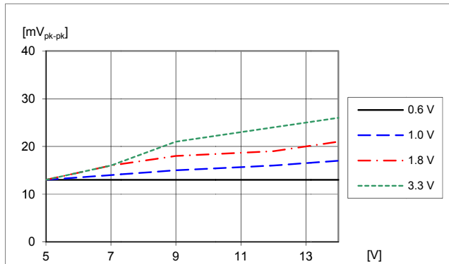
Output voltage ripple V_{pk-pk} at: T_{P1} = +25\text{ }^\circ\text{C} , C_O = 470\text{ }\mu\text{F}/10\text{ m}\Omega , I_O = 40\text{ A} .
