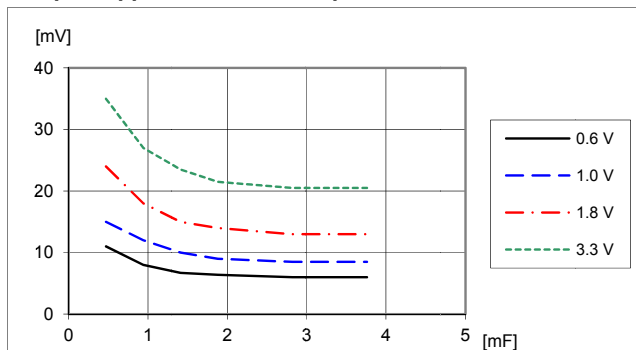
Output voltage ripple V_{pk-pk} at: T_{P1} = +25\text{ }^\circ\text{C} , V_I = 12\text{ V} , I_O = 40\text{ A} . Parallel coupling of capacitors with 470\text{ }\mu\text{F}/10\text{ m}\Omega .
