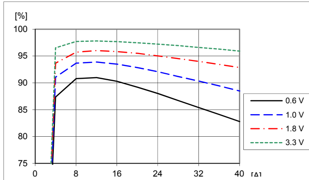
Efficiency vs. Output Current, V_I = 5\text{ V}
