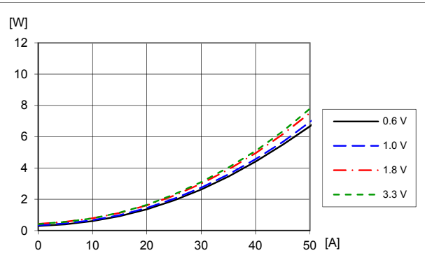
Dissipated power vs. load current and output voltage: T_{P1} = +25\text{ }^\circ\text{C} , V_I = 5\text{ V} , f_{sw} = 320\text{ kHz} , C_O = 470\text{ }\mu\text{F}/10\text{ m}\Omega .
