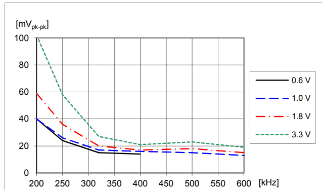
Output voltage ripple V_{pk-pk} at: T_{P1} = +25\text{ }^\circ\text{C} , V_I = 12\text{ V} , C_O = 470\text{ }\mu\text{F}/10\text{ m}\Omega , I_O = 40\text{ A} . Default configuration except changed frequency.
