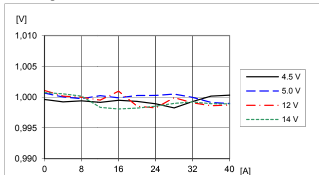
Load regulation at V_O = 1.0\text{ V} at: T_{P1} = +25\text{ }^\circ\text{C} , C_O = 470\text{ }\mu\text{F}/10\text{ m}\Omega
