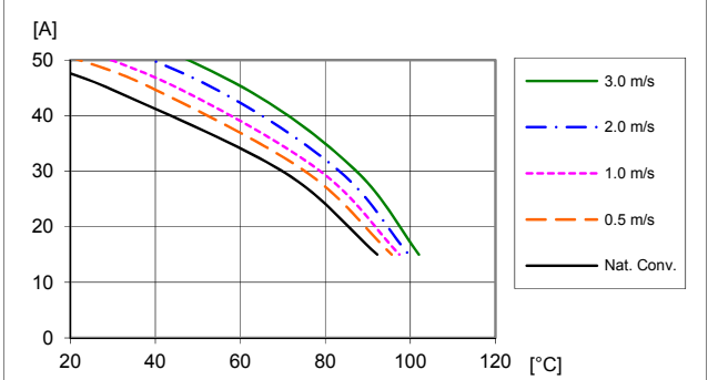
Output Current Derating, V_O = 3.3\text{ V}
