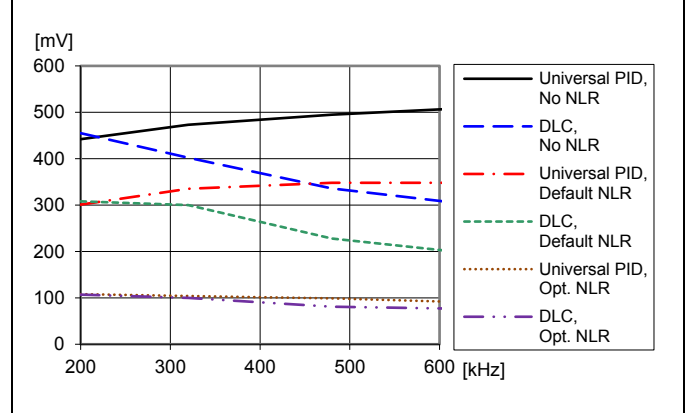
Load transient peak voltage deviation vs. frequency. Step-change (12.5-37.5-12.5 A). T_{P1} = +25^\circ\text{C} , V_I = 12\text{ V} , V_O = 1.0\text{ V} , C_O = 470\text{ }\mu\text{F}/10\text{ m}\Omega
