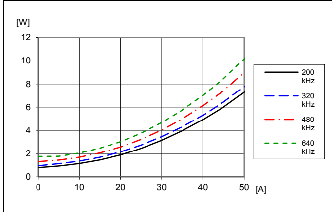
Dissipated power vs. load current and switching frequency at T_{P1} = +25^\circ\text{C} , V_I = 12\text{ V} , V_O = 1.0\text{ V} , C_O = 470\text{ }\mu\text{F}/10\text{ m}\Omega . Default configuration except changed frequency
