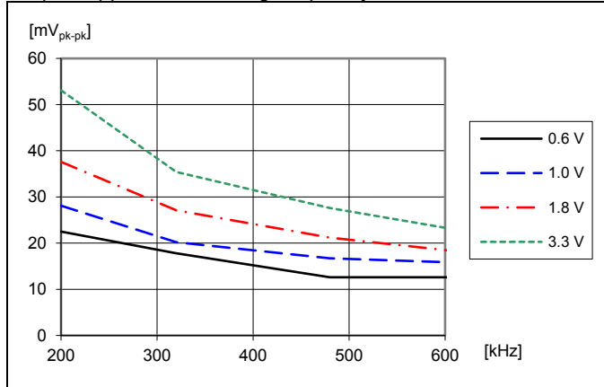
Output voltage ripple V_{pk-pk} at: T_{P1} = +25^\circ\text{C} , V_I = 12\text{ V} , C_O = 470\text{ }\mu\text{F}/10\text{ m}\Omega , I_O = 50\text{ A} resistive load. Default configuration except changed frequency.
