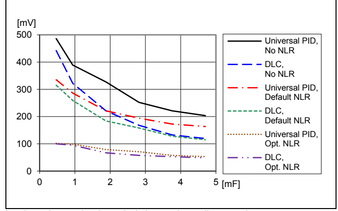
Load transient peak voltage deviation vs. decoupling capacitance. Step (12.5-37.5-12.5 A). Parallel coupling of capacitors with 470\text{ }\mu\text{F}/10\text{ m}\Omega , T_{P1} = +25^\circ\text{C} , V_I = 12\text{ V} , V_O = 3.3\text{ V} , f_{sw} = 320\text{ kHz} , di/dt = 2\text{ A}/\mu\text{s}
