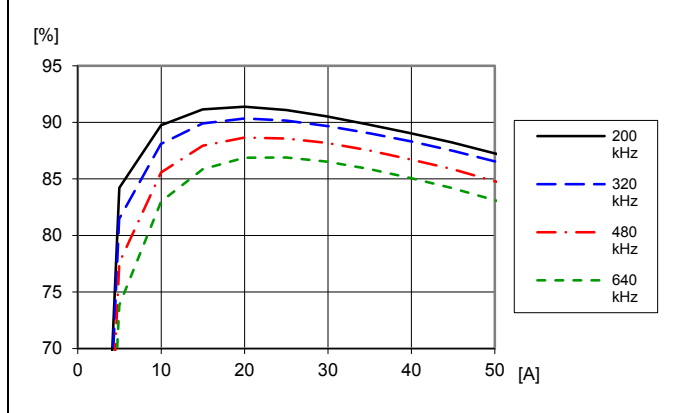
Efficiency vs. load current and switching frequency at T_{P1} = +25^\circ\text{C} , V_I = 12\text{ V} , V_O = 1.0\text{ V} , C_O = 470\text{ }\mu\text{F}/10\text{ m}\Omega . Default configuration except changed frequency
