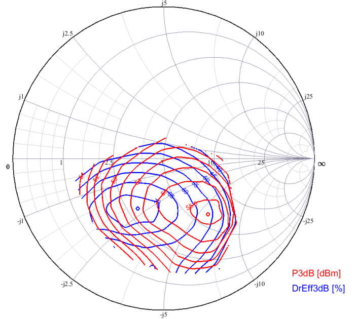
Load Pull at 1.84 GHz
