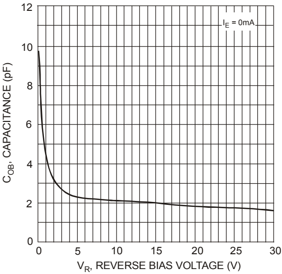
Fig. 9 Output Capacitance
