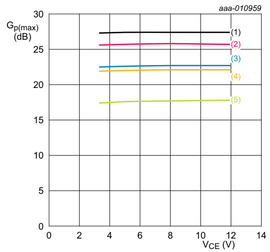
I_C = 10 \text{ mA} ; T_{amb} = 25 \text{ }^\circ\text{C} . If K > 1 then G_{p(max)} = maximum power gain. If K < 1 then G_{p(max)} = MSG. (1) f = 300 \text{ MHz} (2) f = 433 \text{ MHz} (3) f = 800 \text{ MHz} (4) f = 900 \text{ MHz} (5) f = 1800 \text{ MHz}
